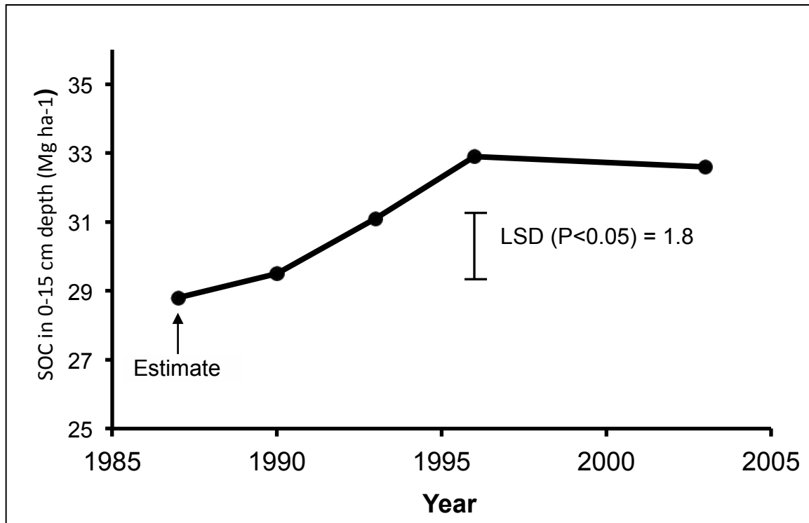
Figure 1. Trends in soil organic carbon (SOC) (1987-2003) averaged over rotations on the New Rotation experiment (redrawn from Campbell 2 ).
